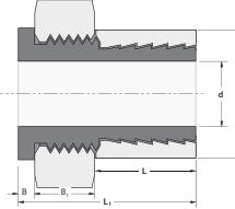
Smooth Bore
